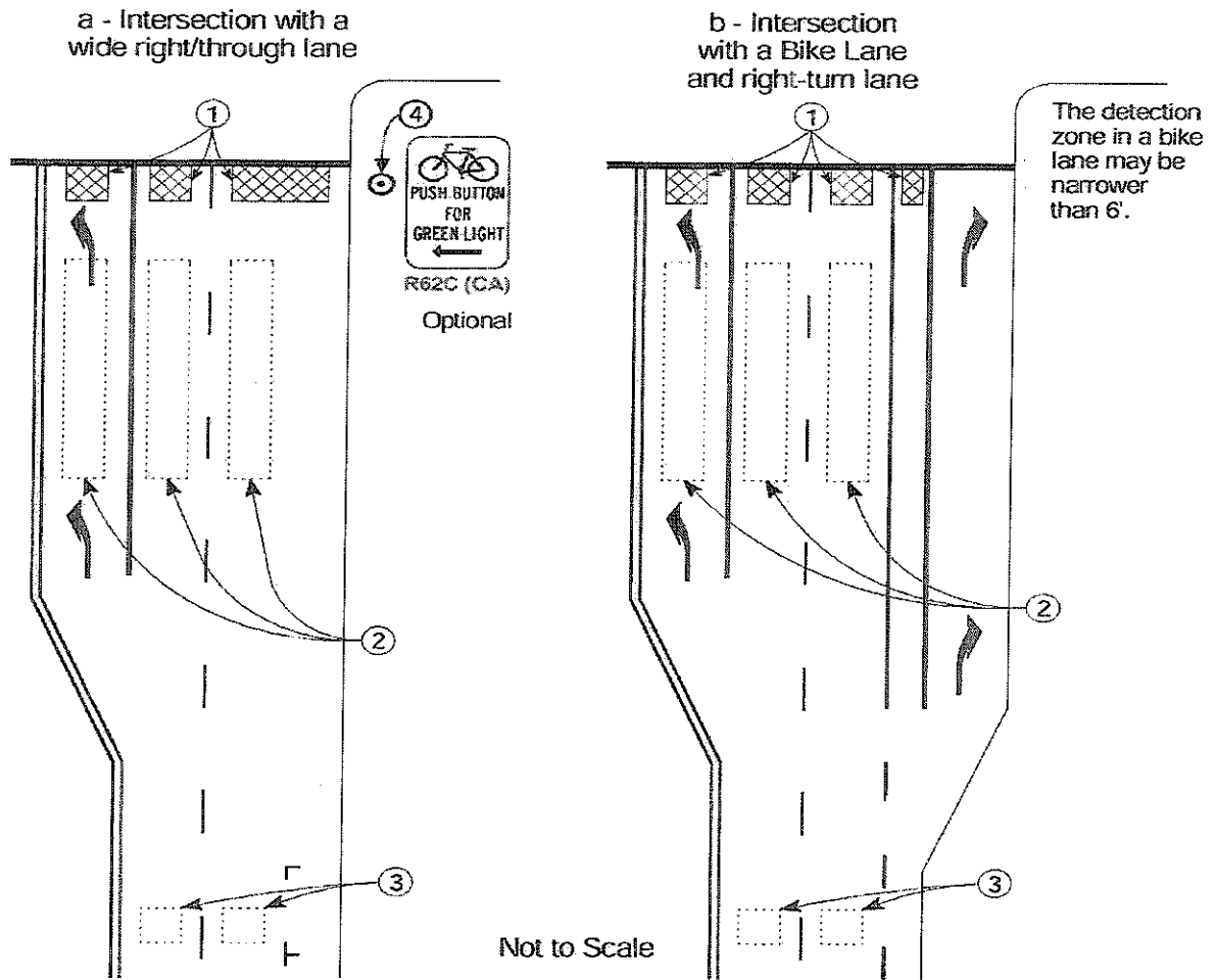
Figure 4D-111(CA) Examples of Detection Systems (Sheet 1 of 3)
